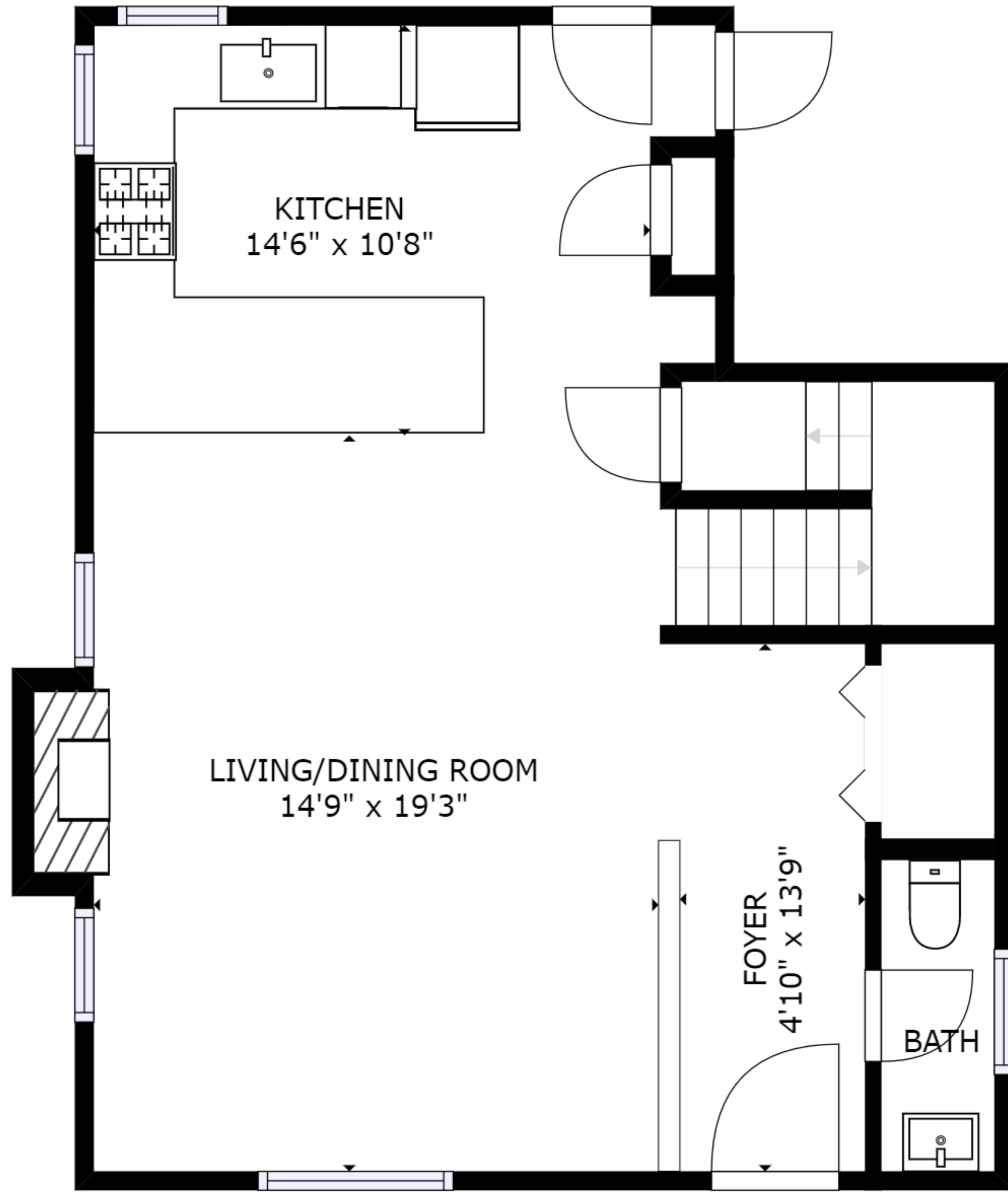
FLOOR 1
